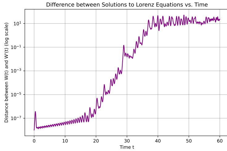
Figure 5: Exponential divergence of the two trajectories. Small perturbations ( \sim 10^{-8} ) grow exponentially with a Lyapunov timescale of approximately 2.5 time units. After t \approx 30 , the trajectories stop correlating.
