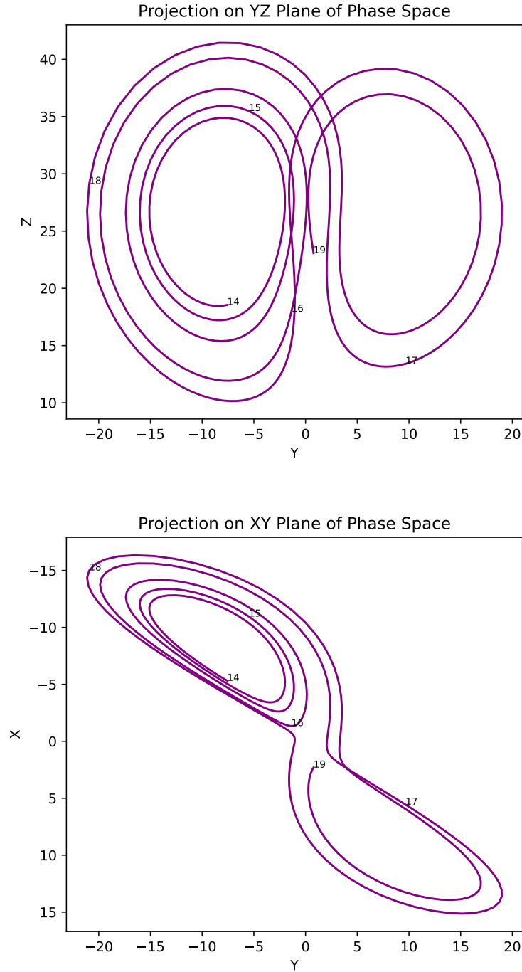
Figure 4: Plot 1 shows the projection of the Lorenz attractor onto the YZ plane. The two lobes of the strange attractor are clearly visible, showing the complex structure visited by the trajectory. Plot 2 shows the projection of the Lorenz attractor onto the XY plane. The characteristic butterfly-like shape emerges from this perspective, illustrating why this structure is sometimes called the “butterfly attractor.” Numbers mark iterations at 100-step intervals.
