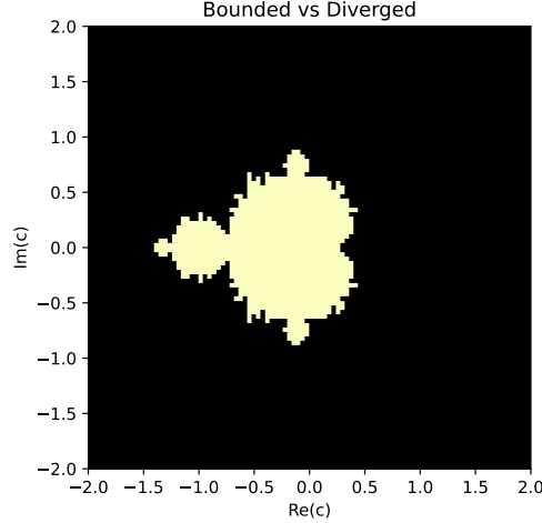
Figure 1: Classification of points in the complex plane as bounded (white) or diverged (black). The Mandelbrot set is clearly visible as the white region.
